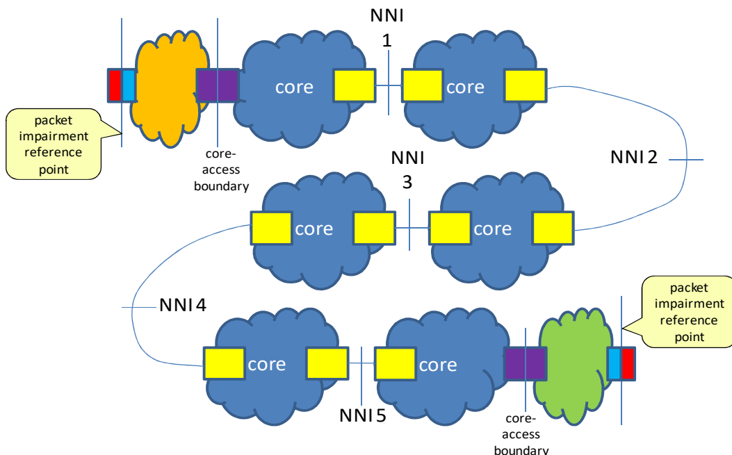
Figure 2: End-to-end IP Connection with Four Transit Networks
