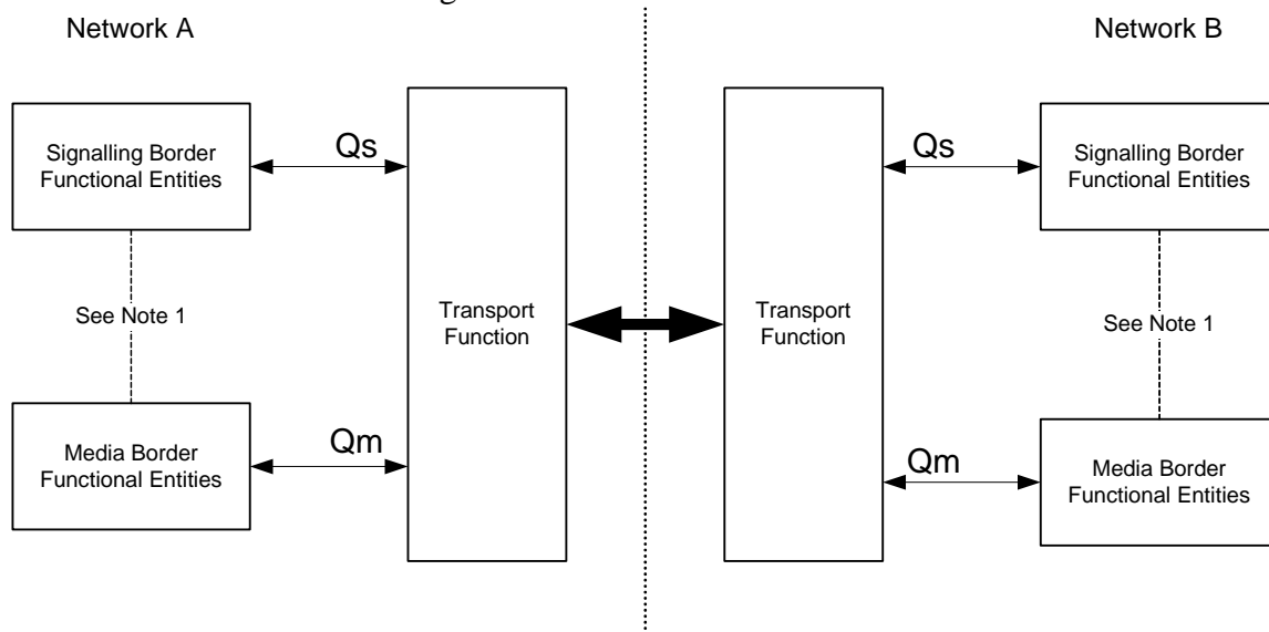
Figure 1 – SIP NNI Functional Model
