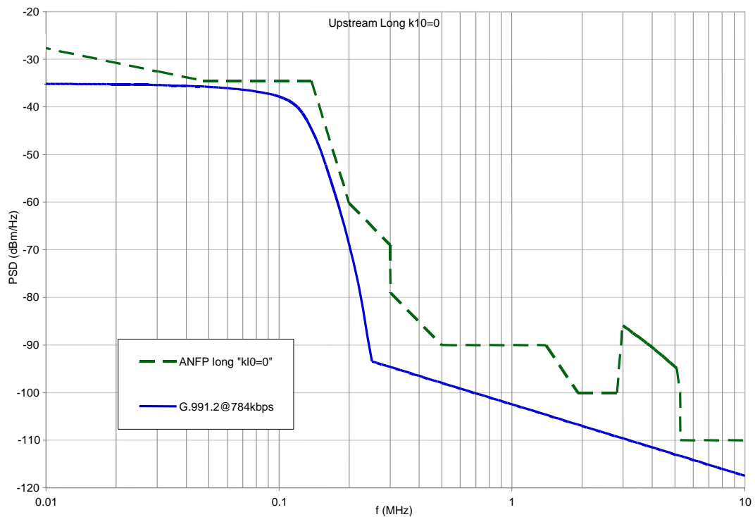
Figure 10 - G.991.2 running at 784kbps versus ANFP Part C (Upstream Long mask)
