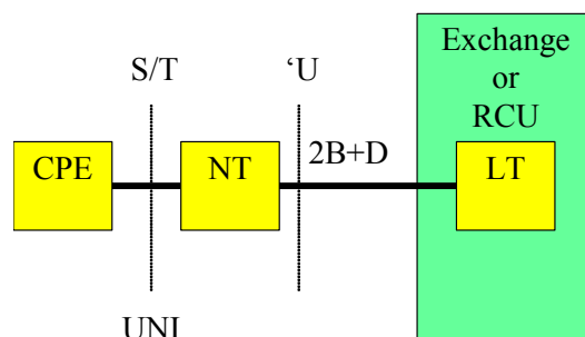
Figure 2 - Basic-rate ISDN-BA concept (DSL)
