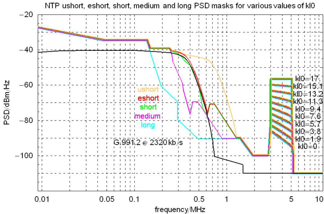
Figure 7 - G.991.2 running at 2320kbps versus ANFP Part C (All Mask)
