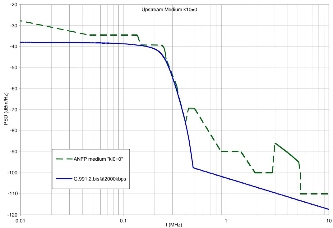
Figure 15 - G.991.2.bis at 2000kbps versus ANFP Part C Upstream Medium Mask (k10=0)
