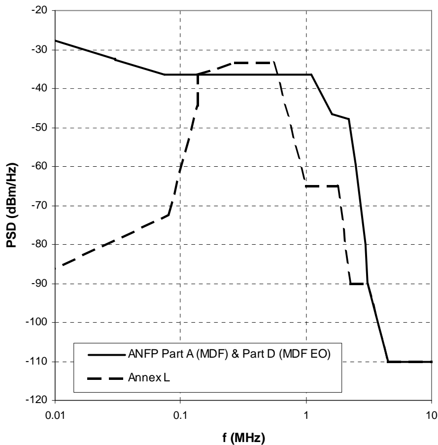
Figure 17 - ANFP Parts A and D PSD mask and ADSL2 Annex L downstream peak PSD mask.
