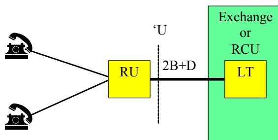
Figure 3 - Two channel digital pair gain (DACs) using ISDN-BA
