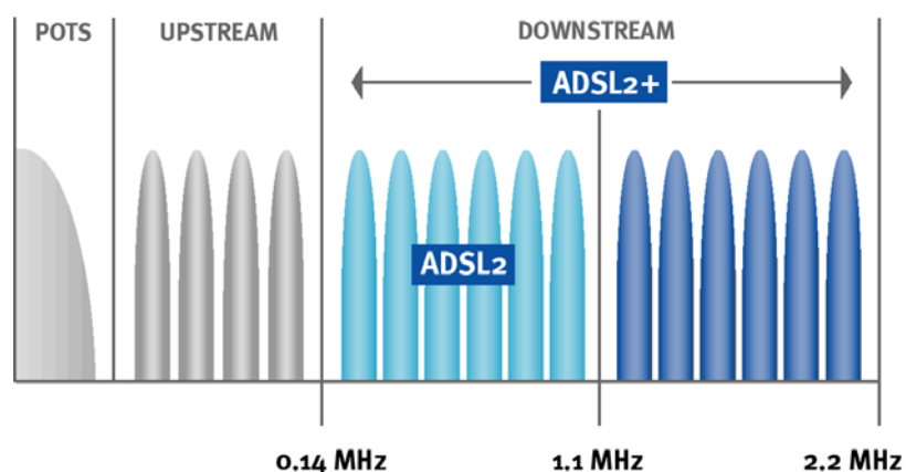
Figure 24 - ADSL2plus doubles the bandwidth used to carry downstream data
