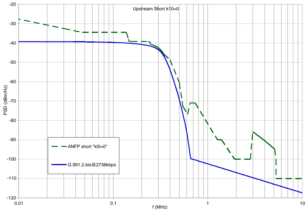
Figure 14 - G.991.2.bis at 2736kbps versus ANFP Part C Upstream Short Mask (k10=0)
