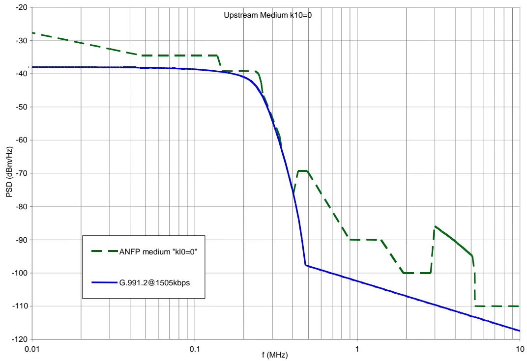
Figure 9 - G.991.2 running at 1505kbps versus ANFP Part C (Upstream Medium mask)
