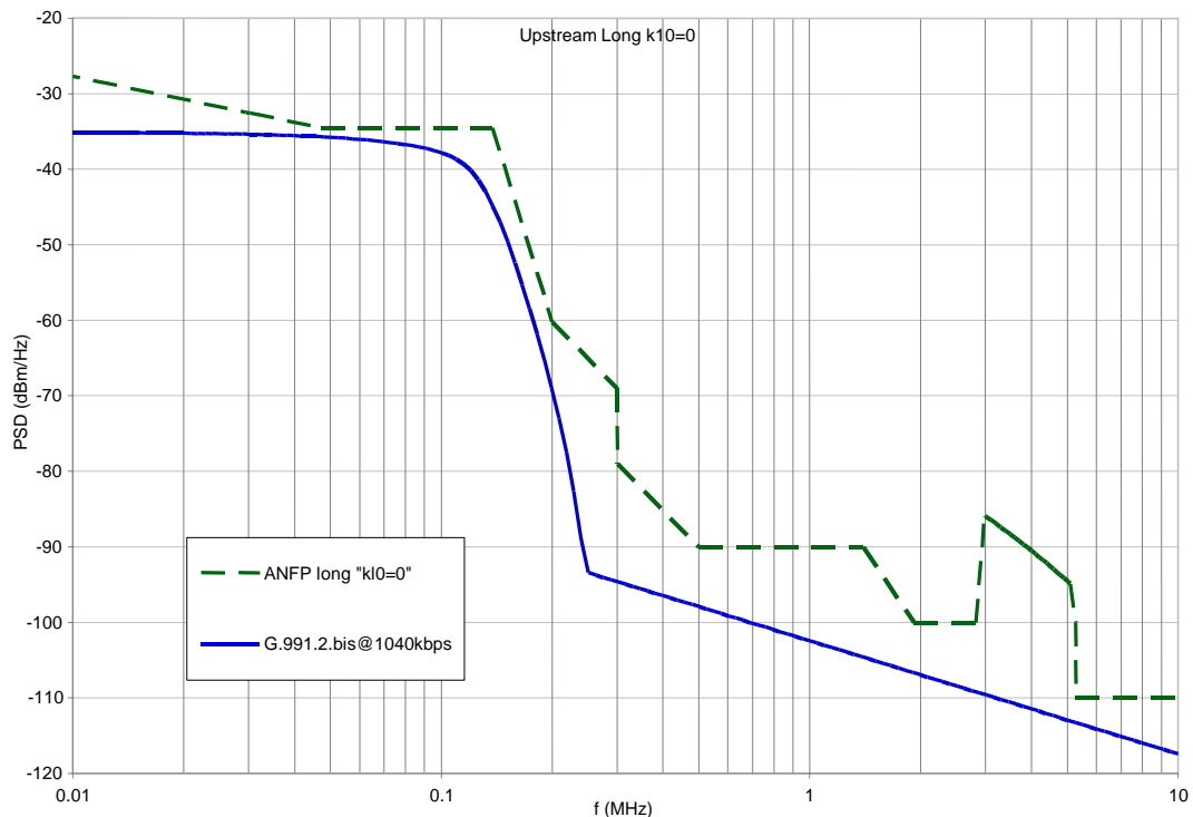
Figure 16 - G.991.2.bis at 1040kbps versus ANFP Part C Upstream Long Mask (k10=0)
