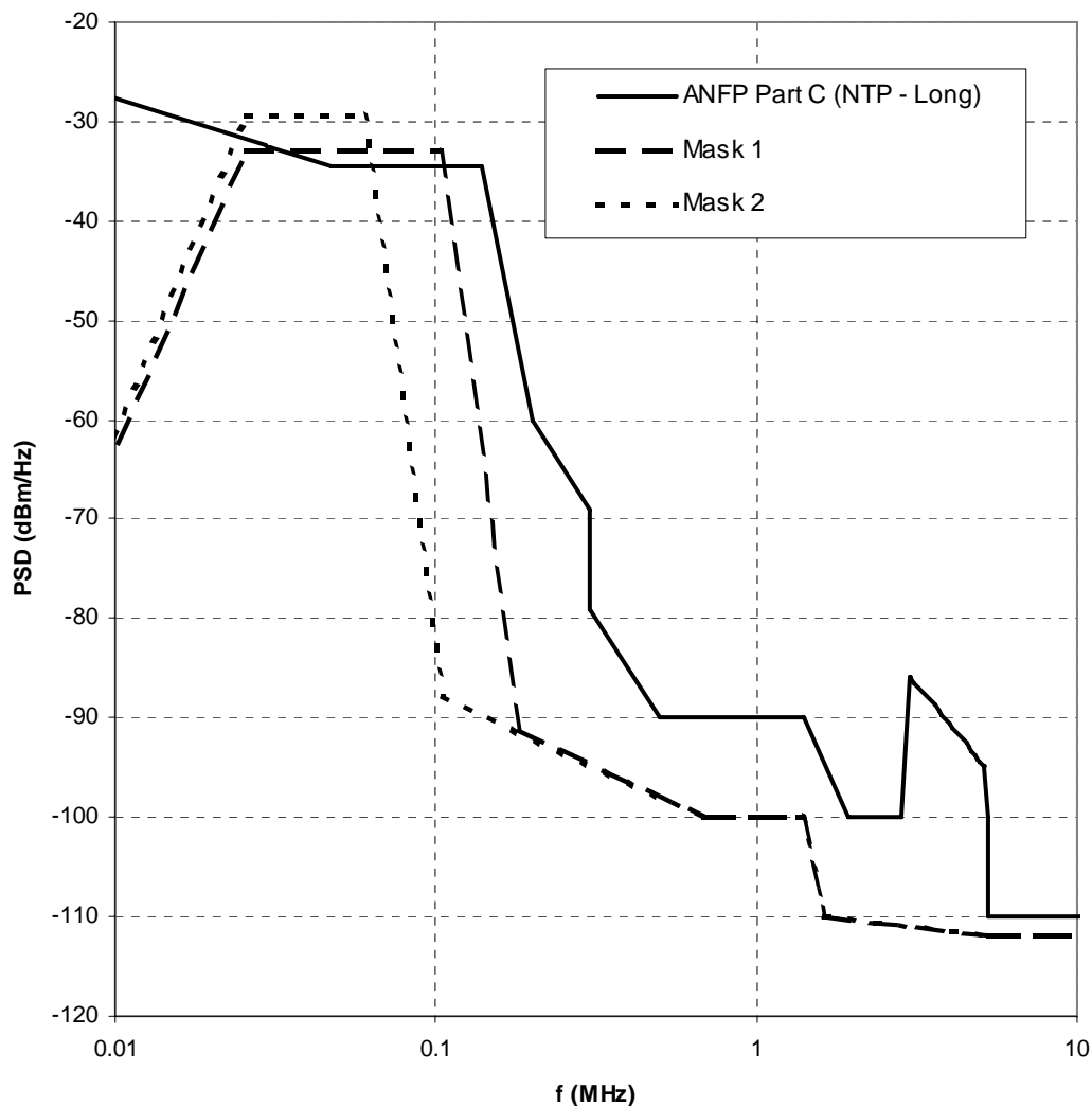
Figure 22 - ANFP Part C - long PSD mask using k_{10}=0 and ADSL2 Annex L peak PSD.
