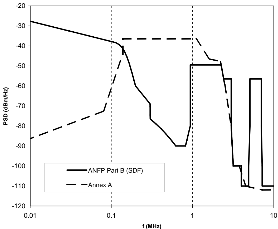
Figure 25 - ANFP Part B PSD mask with CAL = 40 and ADSL2+ Annex A downstream peak PSD mask.
