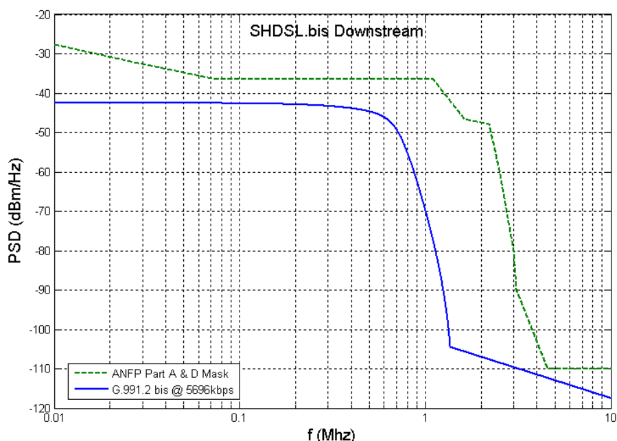
Figure 11 - G.991.2.bis running at 5696kbps versus ANFP Part A and Part D PSD Masks
