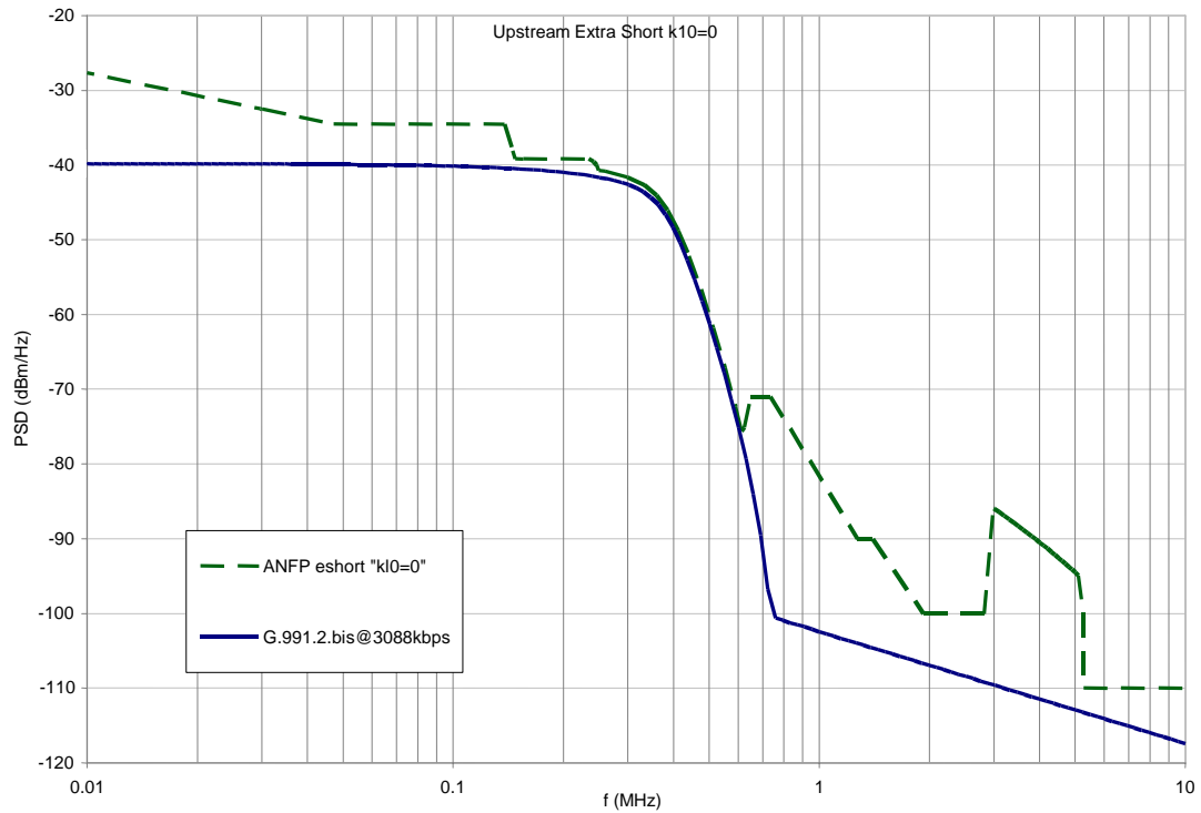
Figure 13 - G.991.2.bis at 3088kbps versus ANFP Part C Upstream Extra Short Mask (k10=0)
