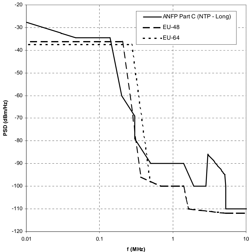
Figure 20 - ANFP Part C - long PSD mask using K10=0 and ADSL2 Annex J EU-48 and EU-64 peak PSD.
