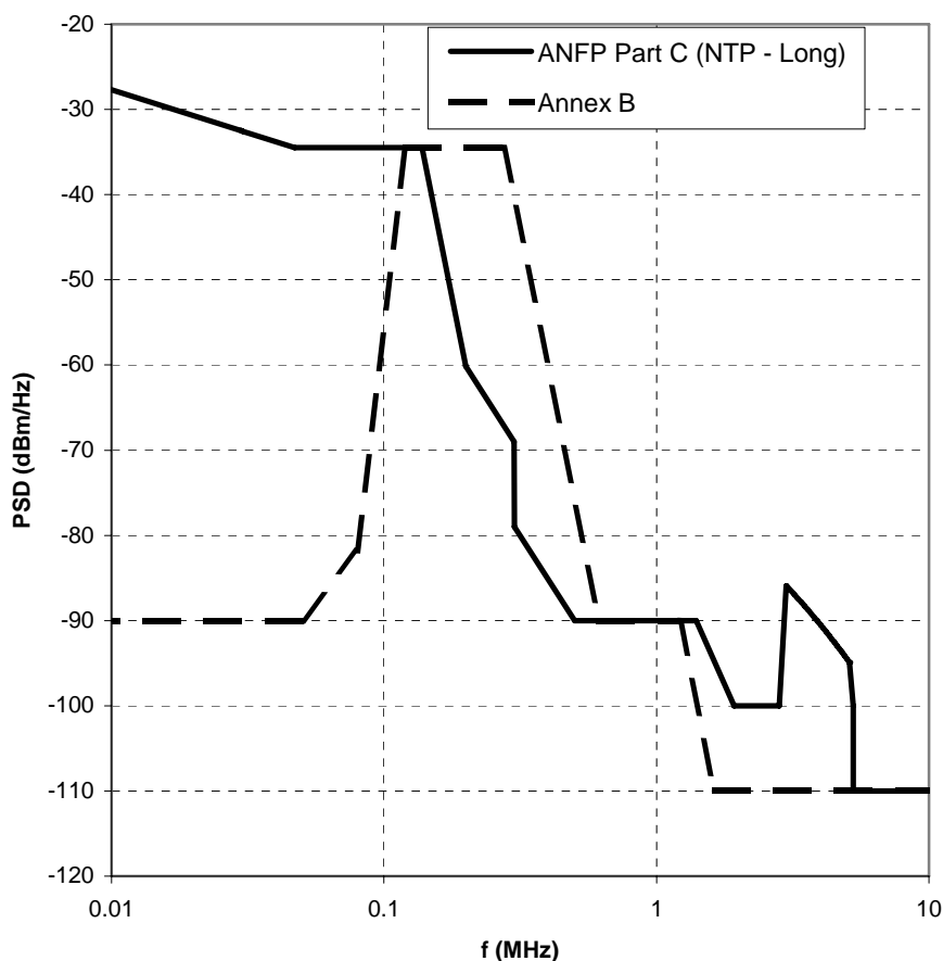
Figure 19 - ANFP Part C - long PSD mask using k10=0 and ADSL2 Annex B peak PSD.
