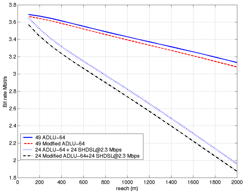
Figure 21 - ADSL upstream bit rate with 49 self-disturbers and with 24 ADSL + 24 SHDSL at 2.3 Mbit/s.
