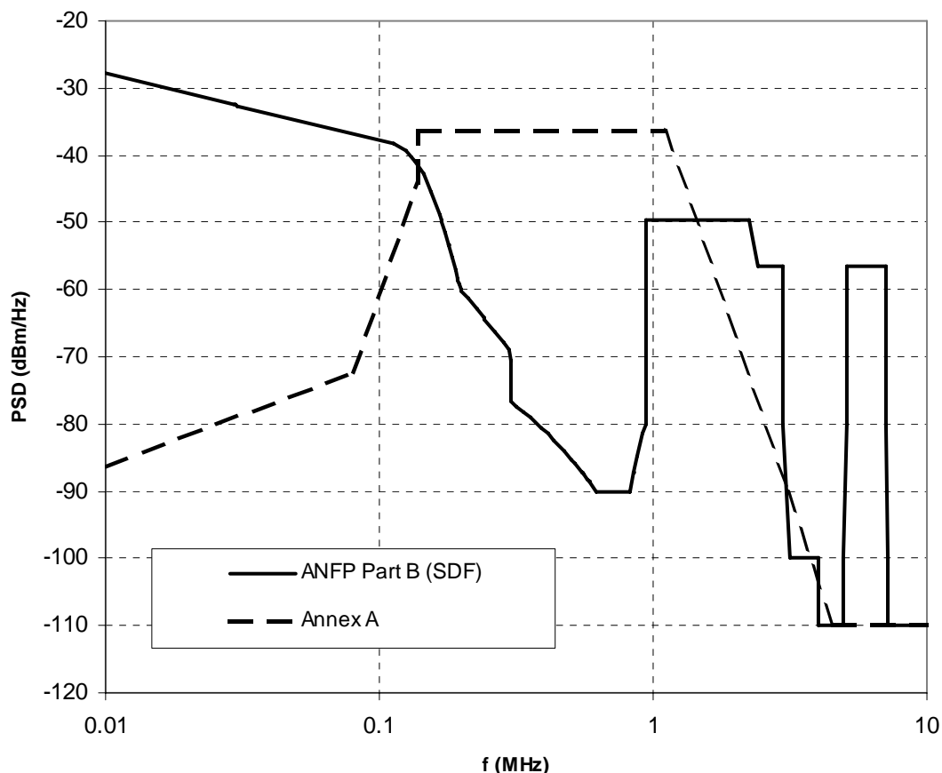
Figure 18 - ANFP Part B PSD mask with CAL = 40 and ADSL2 Annex A downstream peak PSD mask.
