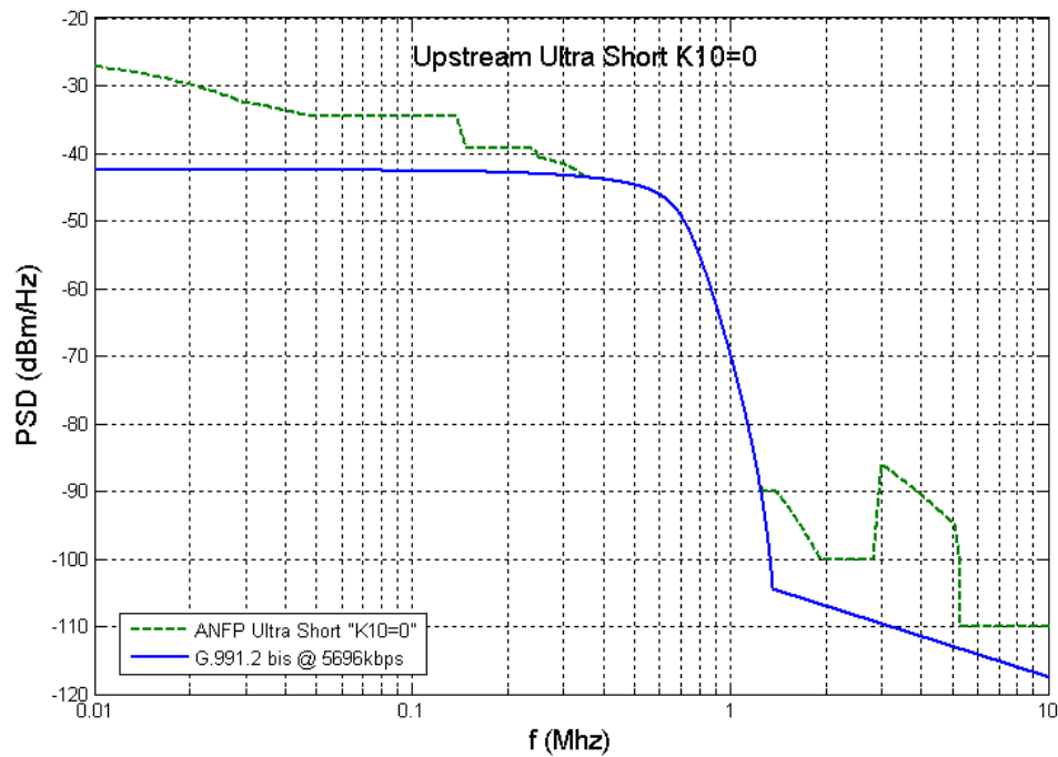
Figure 12 - G.991.2.bis at 5696 kbps versus ANFP Part C Upstream Ultra Short Mask (k10=0)
